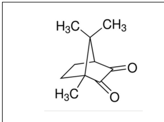
Chemical structure:
